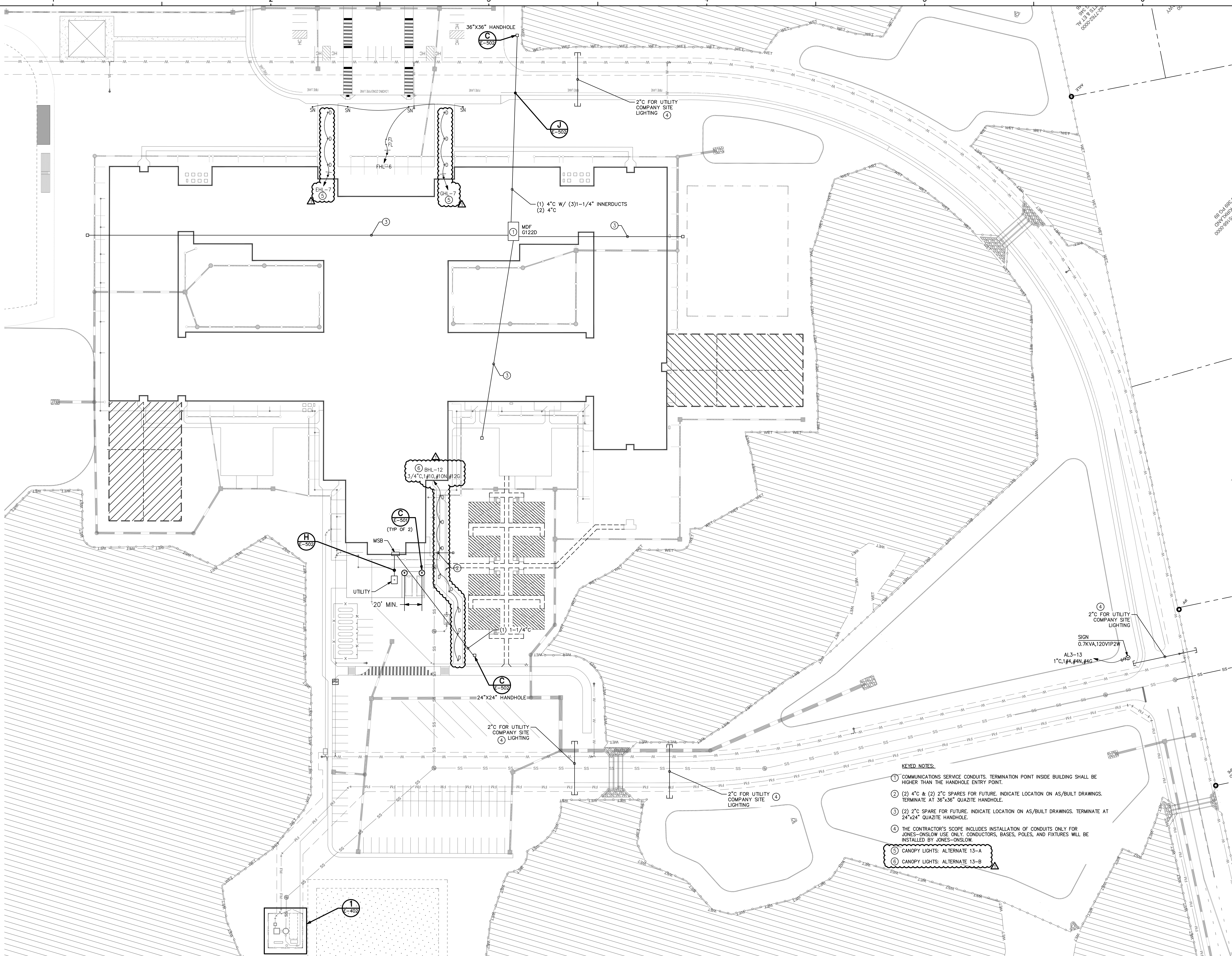
1 ELECTRICAL SITE PLAN SCALE: 1" = 40'-0"
