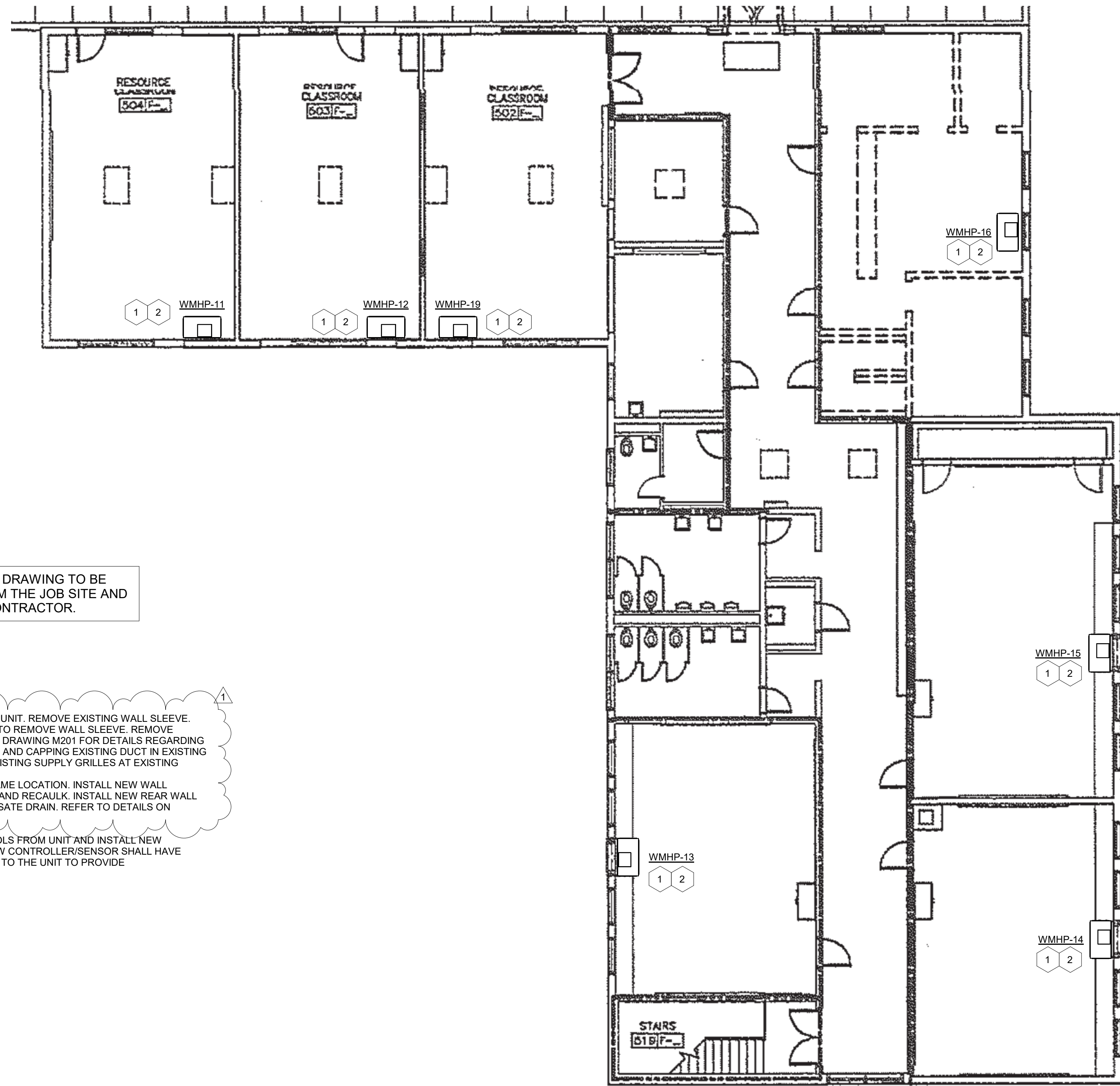
1 HVAC Plan - Area C Upper Level 1/8" = 1'-0"
