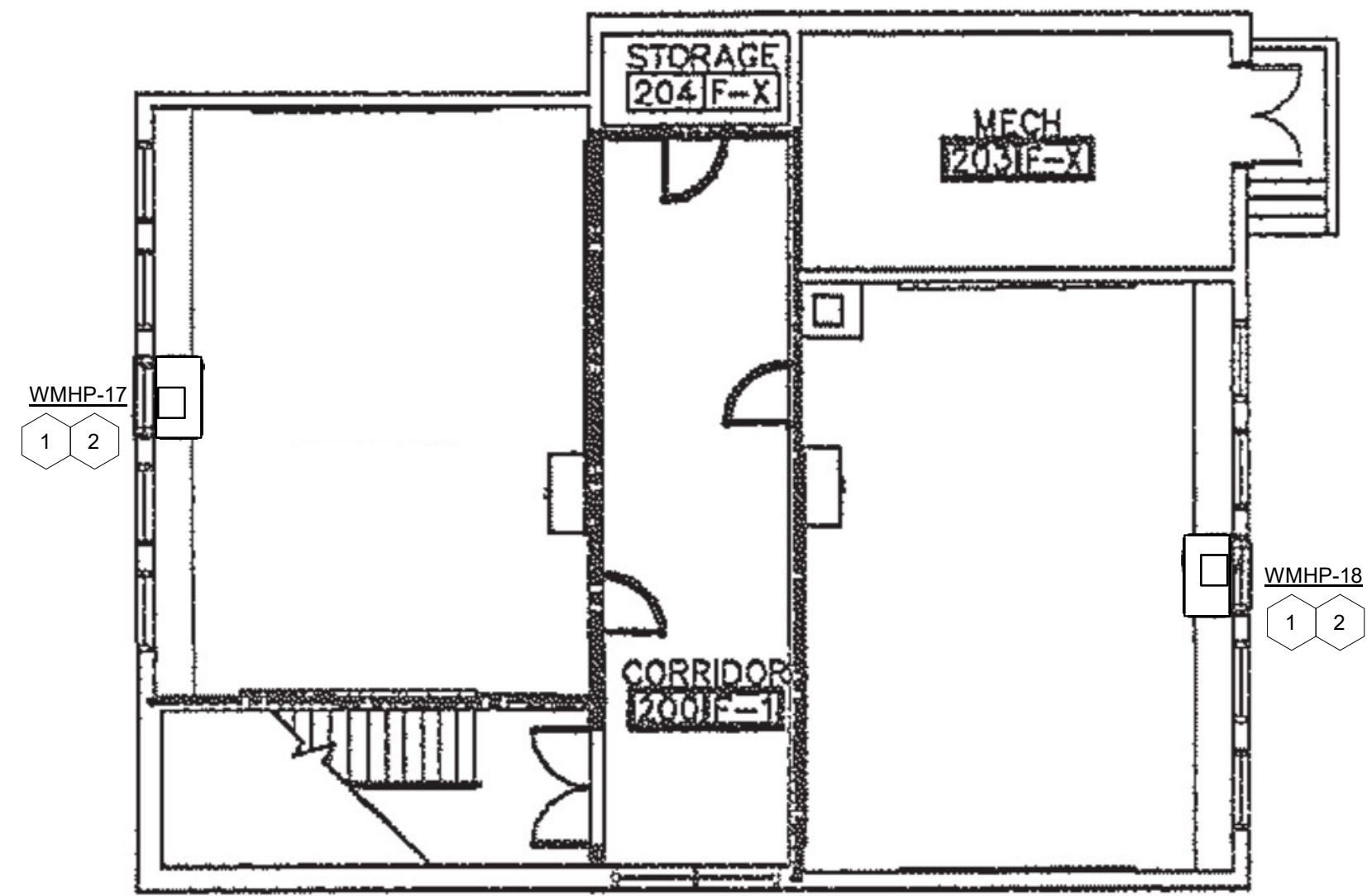
3 HVAC Plan - Area C Lower Level 1/8" = 1'-0"
