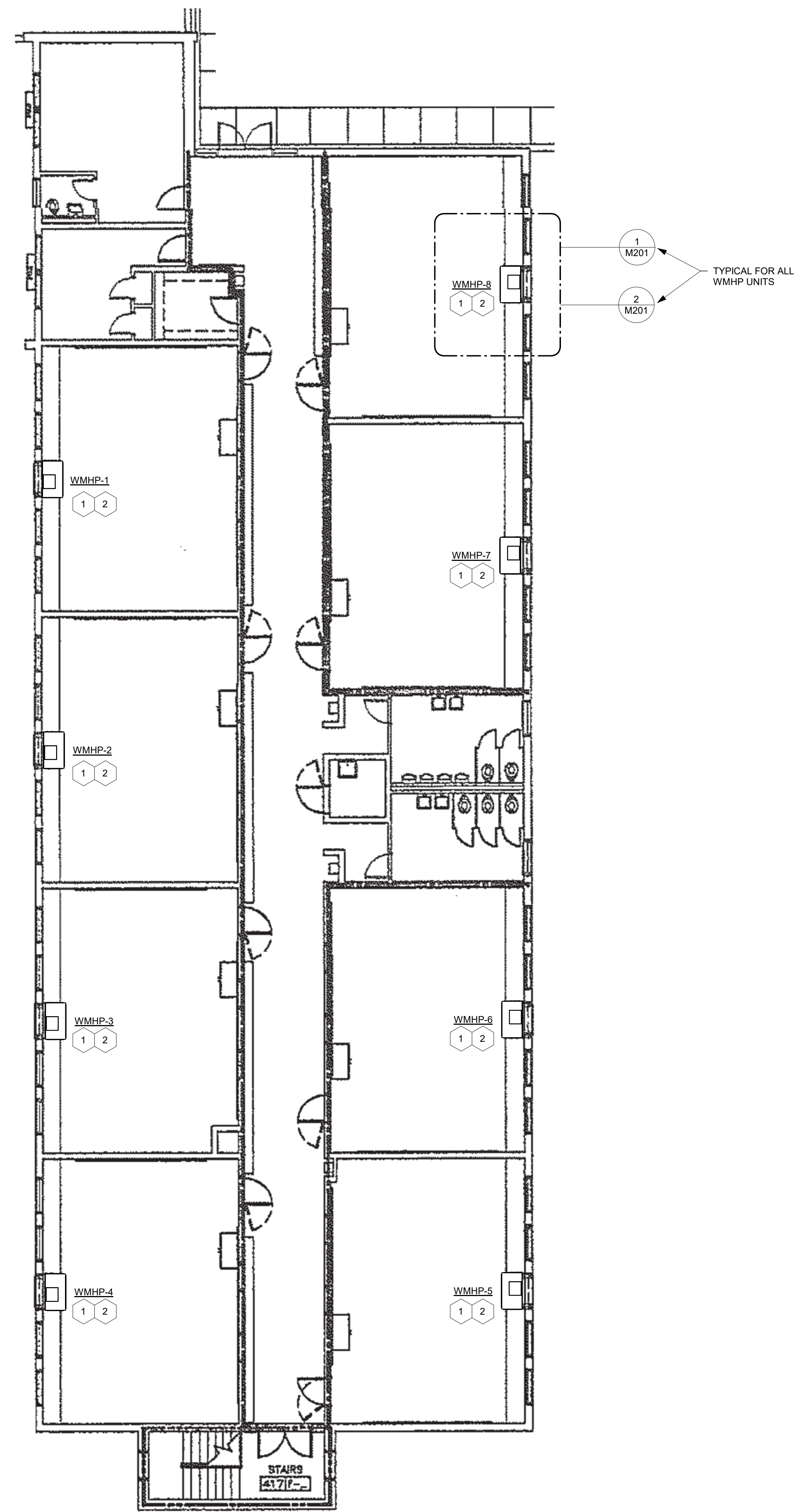
2 HVAC Plan - Area D Upper Level 1/8" = 1'-0"
