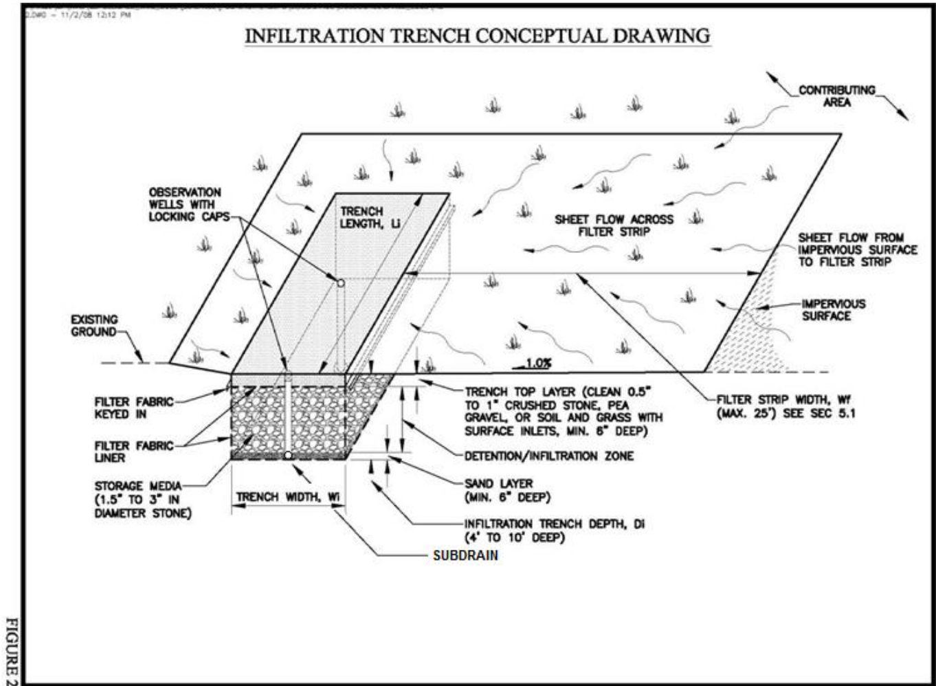
Figure 2 – Infiltration Trench Conceptual Drawing
