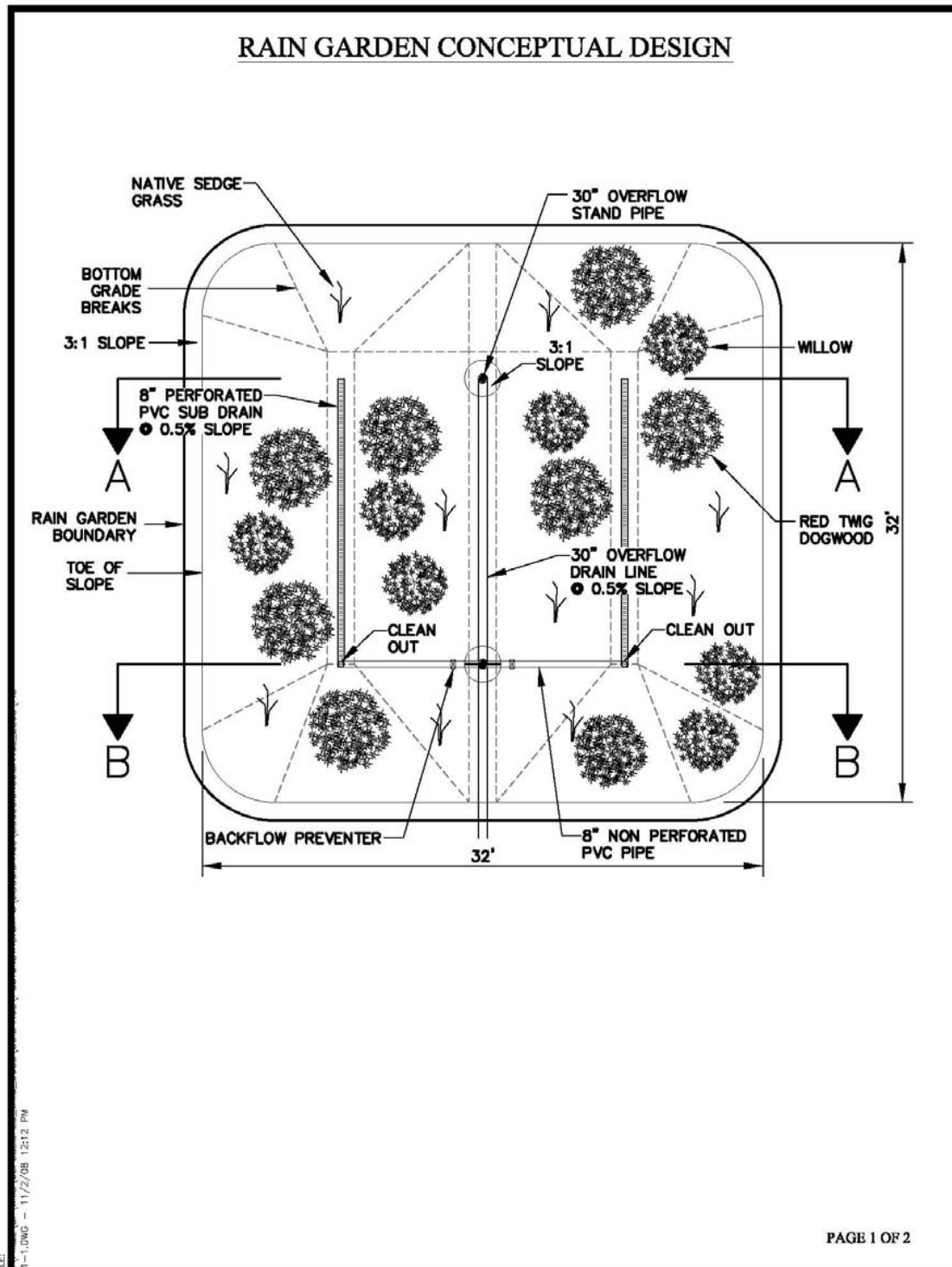
Figure C.1 – Bioretention cell Design Example Page 1
