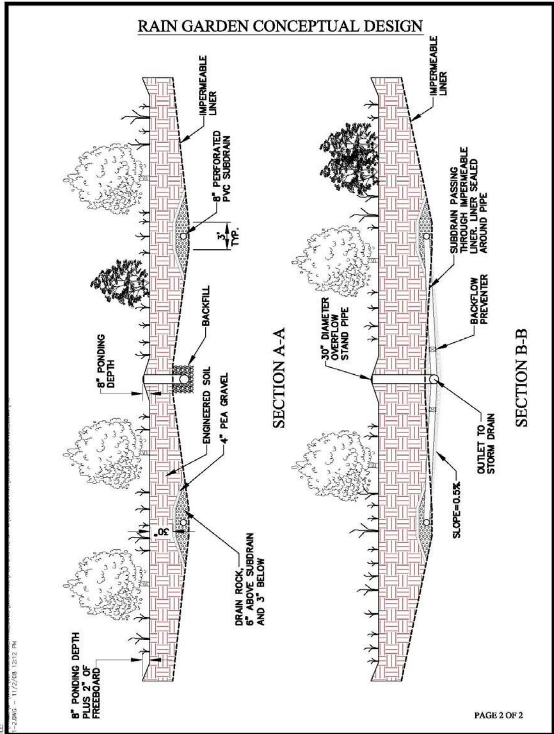
Figure C.1 – Bioretention cell Design Example Page 2
