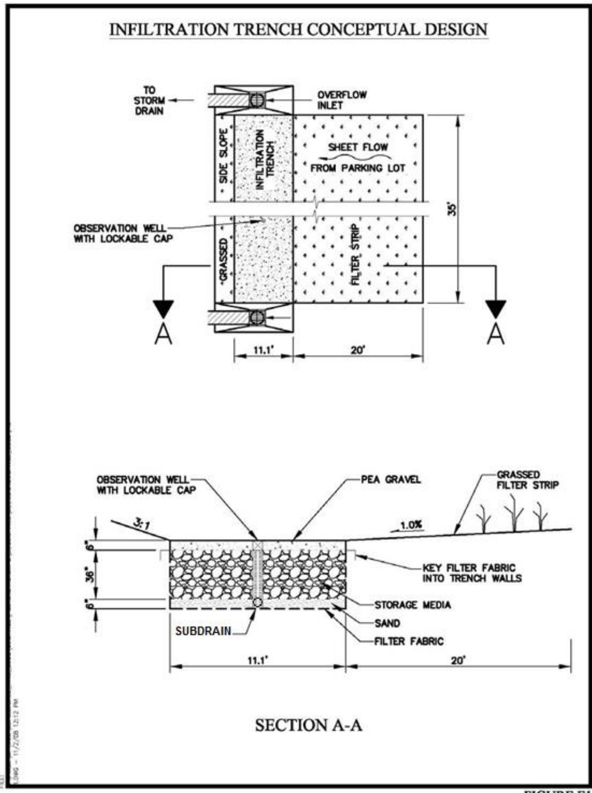
Figure D.1 – Infiltration Trench Design Example
