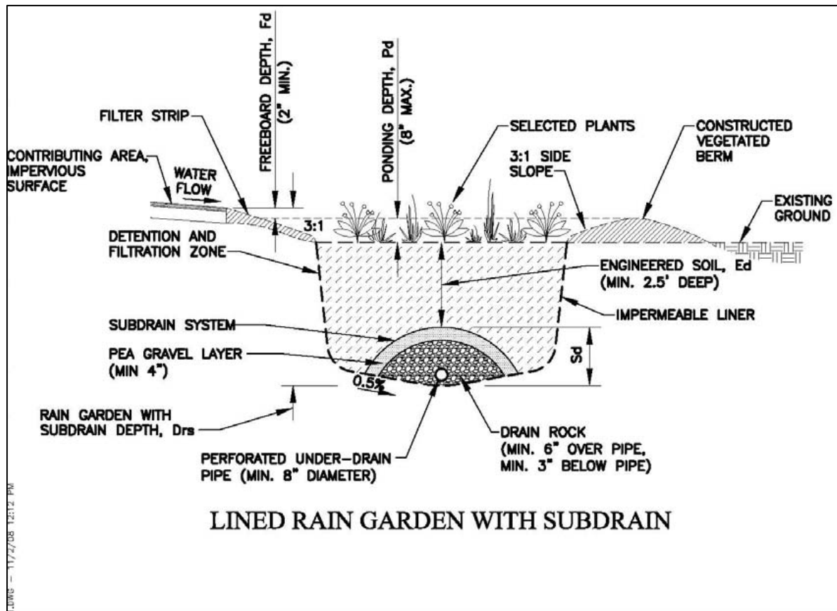
Figure 1 – Conceptual Bioretention Cell Profiles
