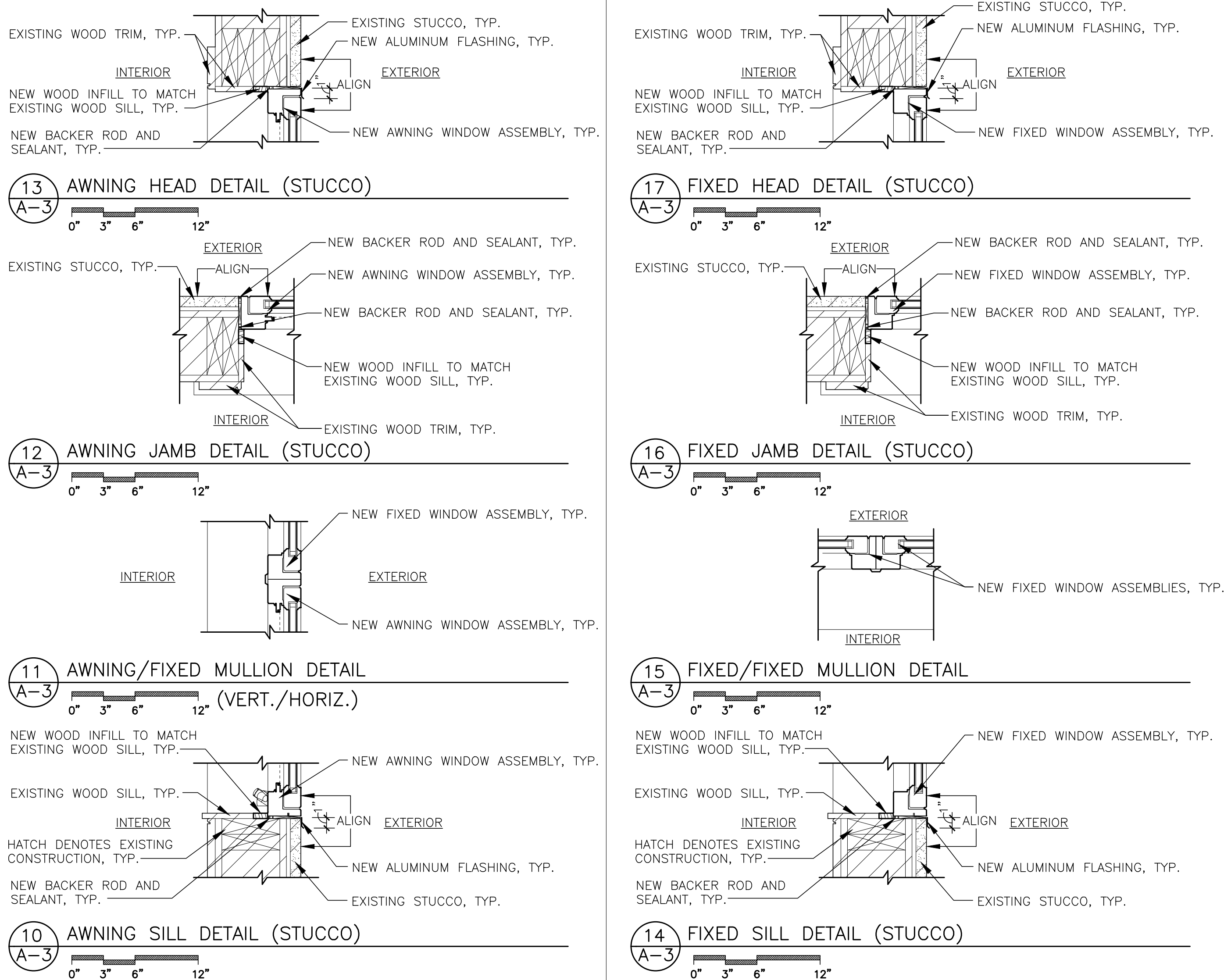
AWNING WINDOW DETAILS (STUCCO)
