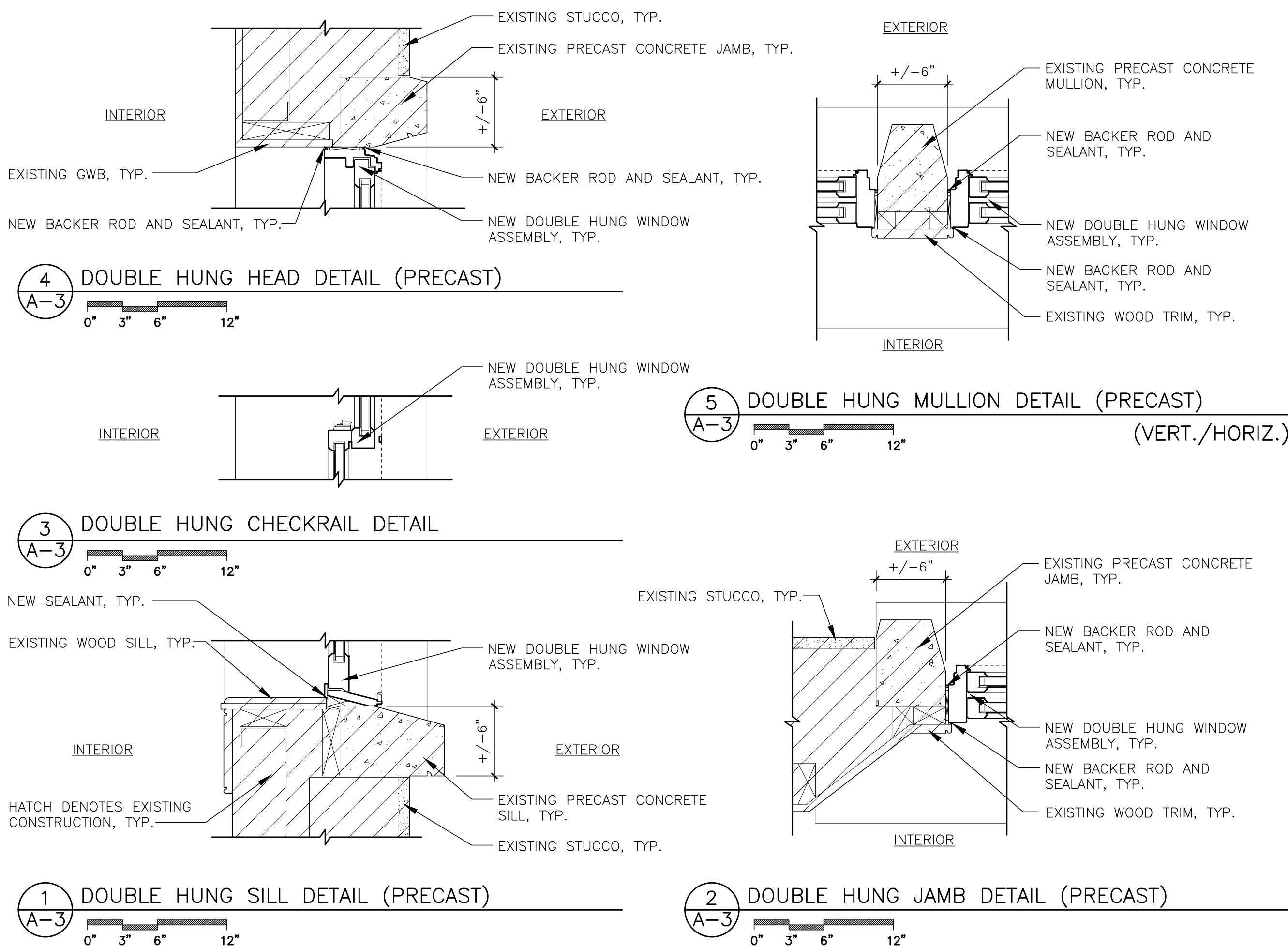
DOUBLE HUNG WINDOW DETAILS (PRECAST)
