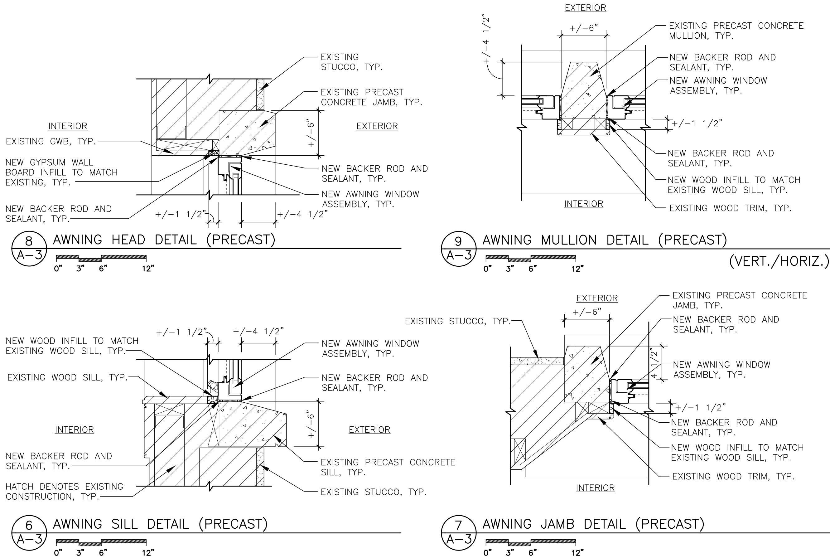
AWNING WINDOW DETAILS (PRECAST)
