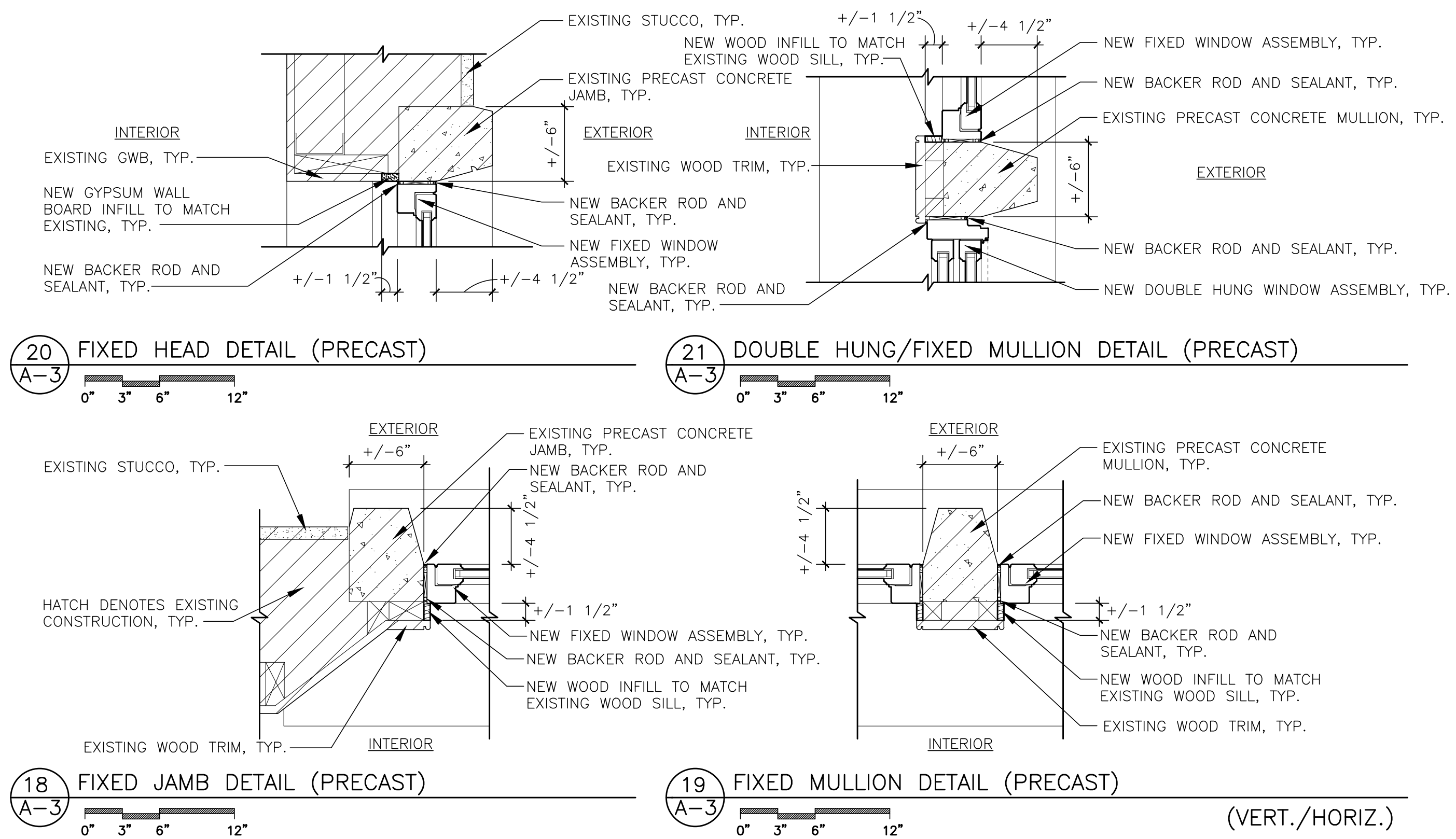
FIXED WINDOW DETAILS (PRECAST)
