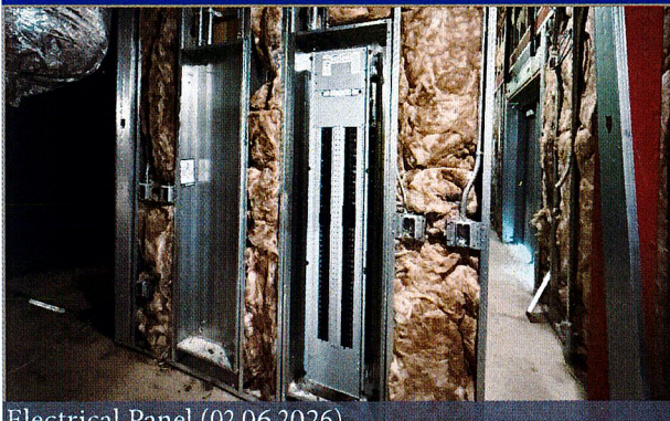
Electrical Panel (02.06.2026)
