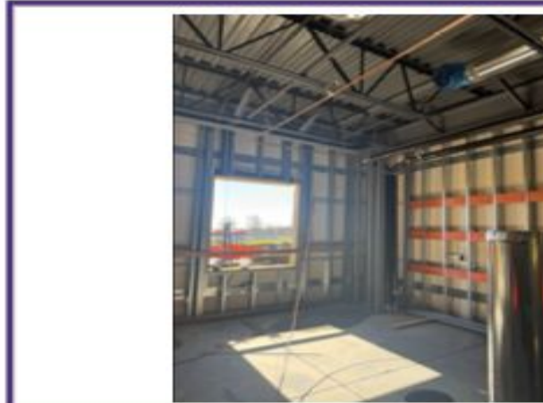
Sheathing and Blocking Complete
