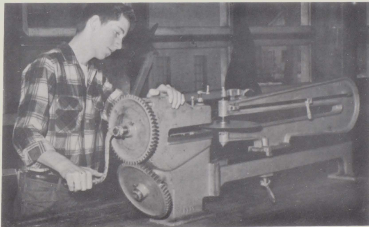
Wayne Foster is operating the ring and circular shears. This machine makes circles of all sizes.
