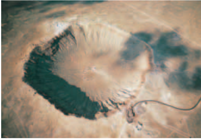
Figure 20 Meteorites occasionally strike Earth's surface. A large meteorite struck Arizona, forming a crater about 1.2 km in diameter and about 200 m deep.
